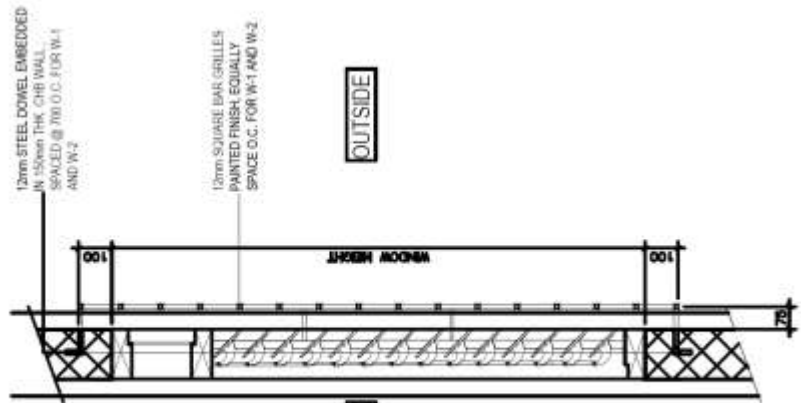
GRILLES DETAIL
