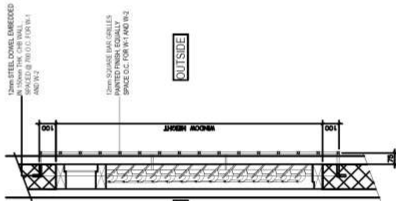
GRILLES DETAIL
